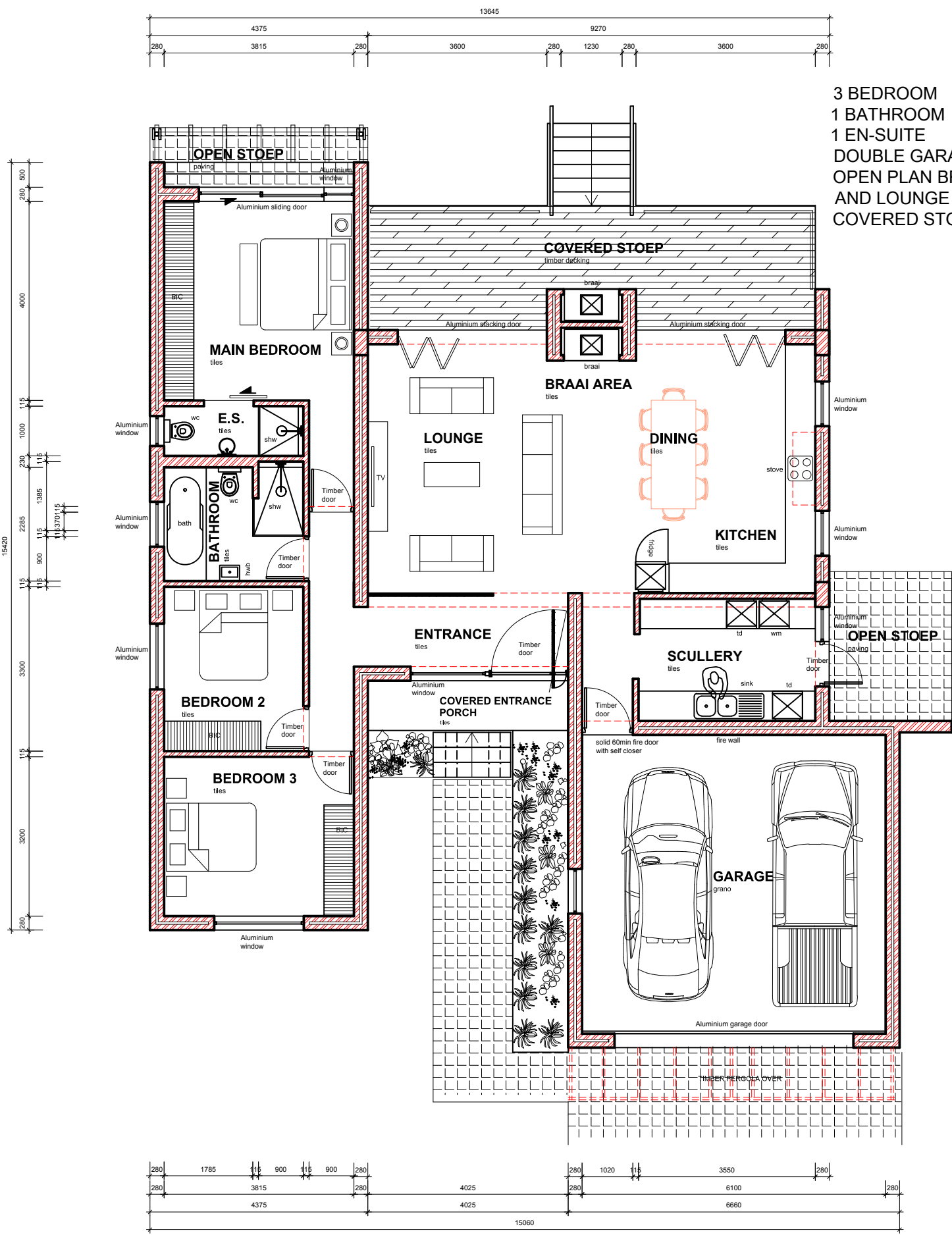
TYPE 13A GROUND STOREY PLAN 1:100
